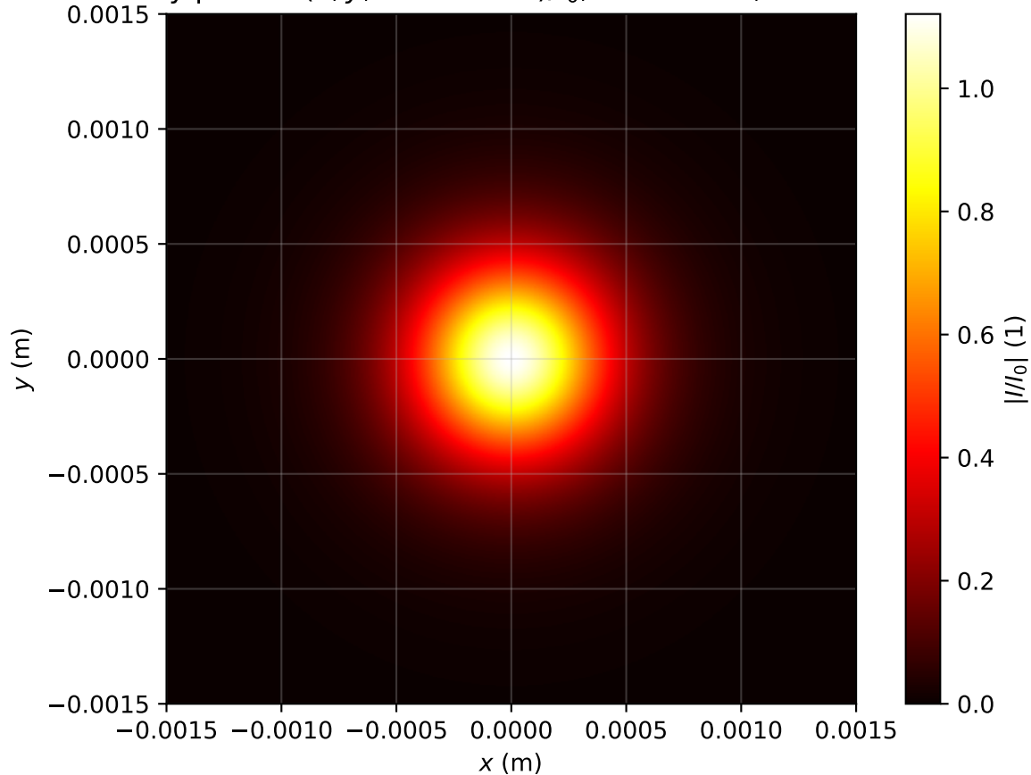
Intensity profile I(x, y, z = 1.911m)/I_0 , P_{in}=0.7P_{cr} , artificial time
